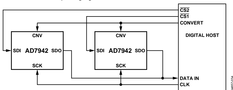
Figure 34. \overline{CS} Mode 4-Wire, No Busy Indicator Connection Diagram
