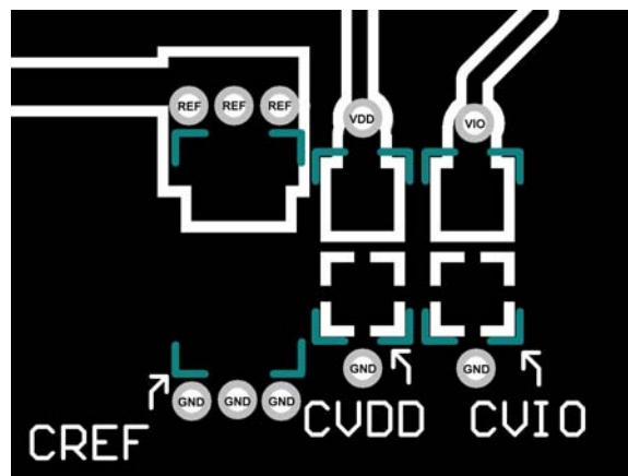
Figure 43. Example of Layout of the AD7942 (Bottom Layer)
