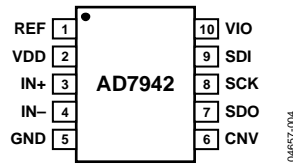
Figure 4.10-Lead MSOP and QFN 1 (LFCSP) Pin Configuration
