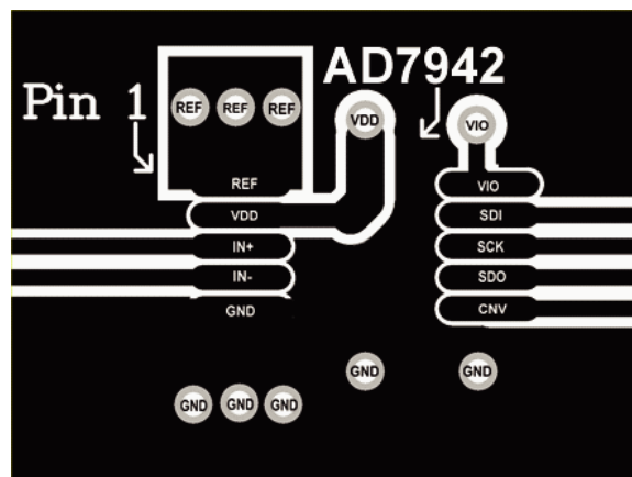
Figure 42. Example of Layout of the AD7942 (Top Layer)
