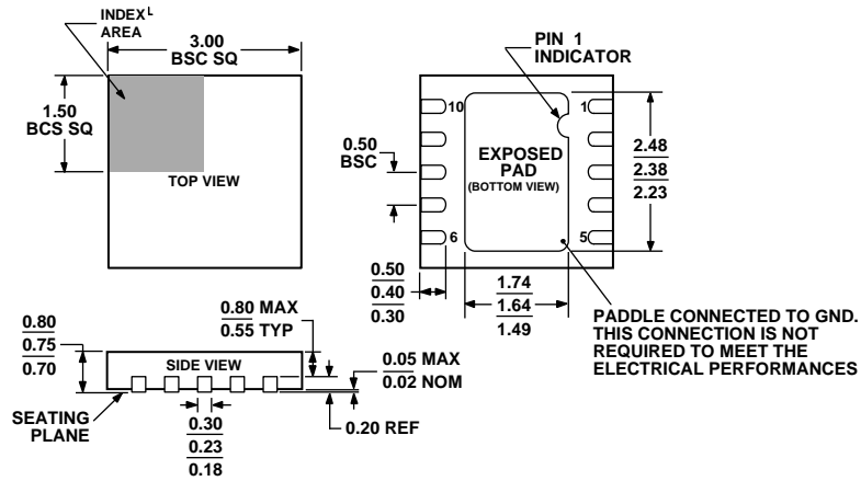
Figure 45. 10-Lead Lead Frame Chip Scale Package [QFN 1 (LFCSP)] 3 mm x 3 mm Body (CP-10) Dimensions shown in millimeters
