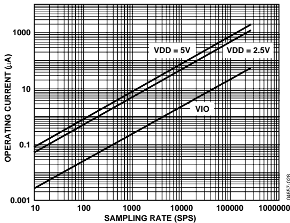
Figure 28. Operating Currents vs. Sampling Rate
