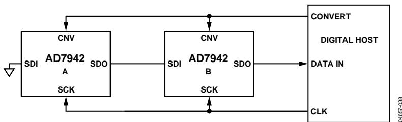
Figure 38. Chain Mode, No Busy Indicator Connection Diagram
