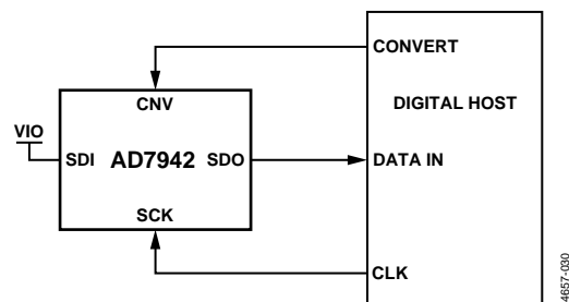
Figure 30. \overline{CS} Mode 3-Wire, No Busy Indicator Connection Diagram (SDI High)
