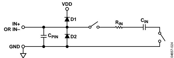
Figure 24. Equivalent Analog Input Circuit
