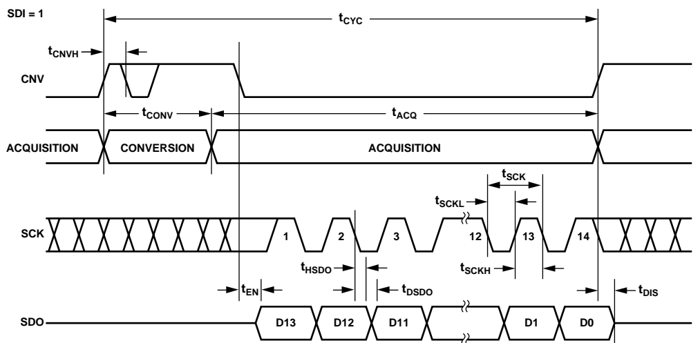
Figure 31. \overline{CS} Mode 3-Wire, No Busy Indicator, Serial Interface Timing (SDI High)
