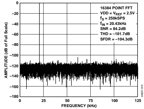
Figure 10. FFT Plot
