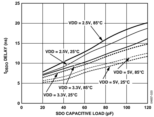
Figure 20. t_{SDO} vs. Capacitance Load and Supply
